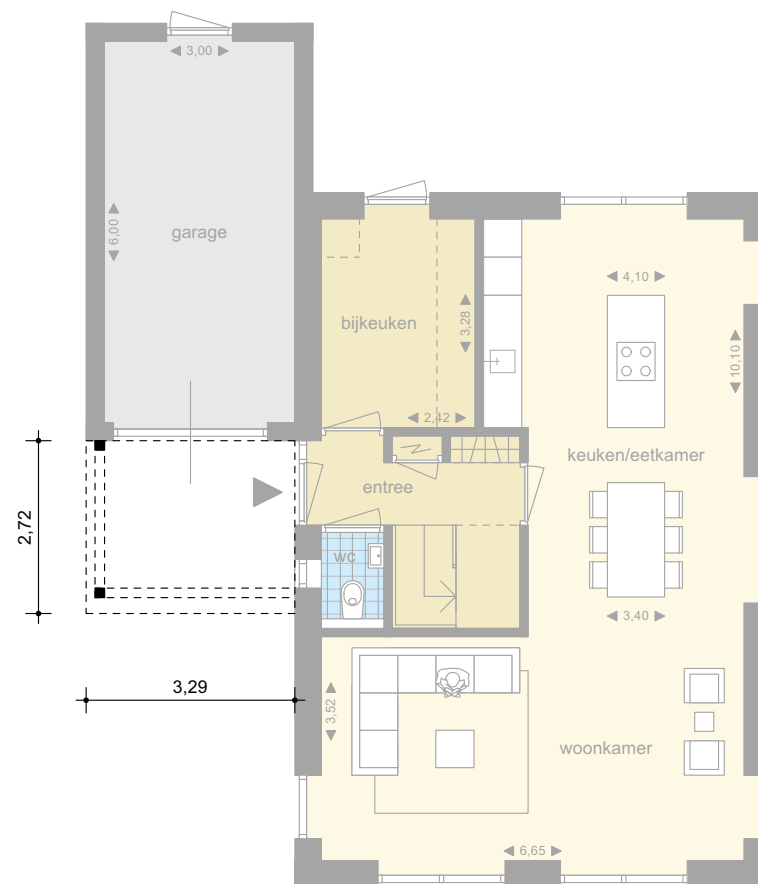
Type 2 - 2,72 m lang
