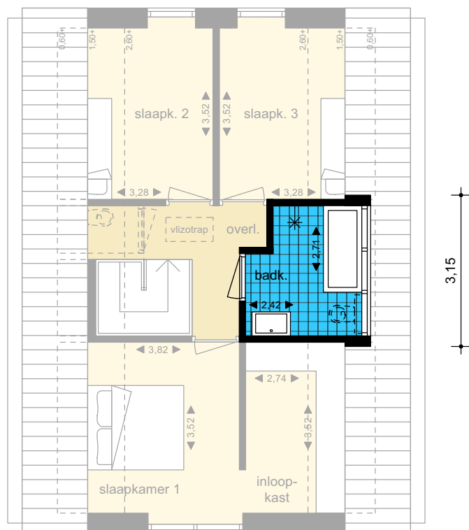
type 2 - dakkapel
